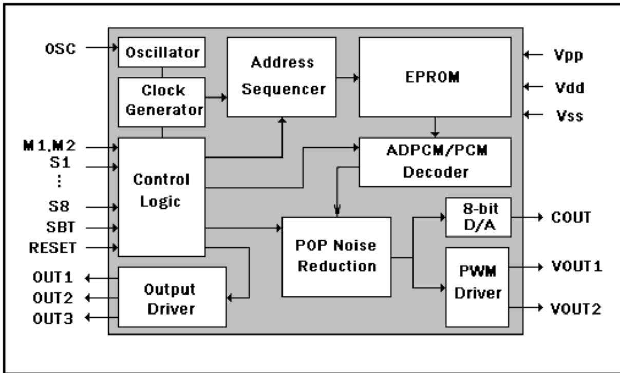
Fig. 17 Block Diagram
