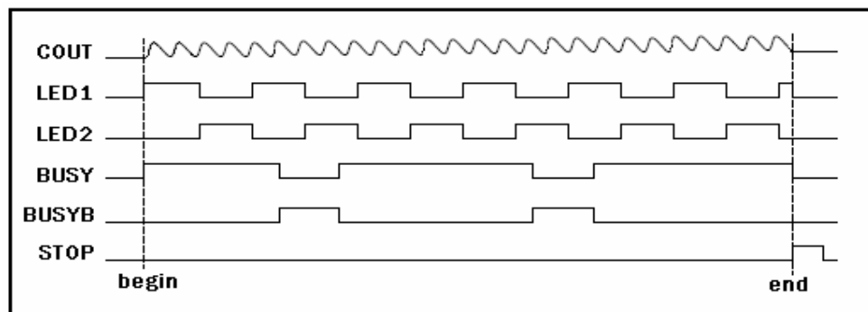
Fig. 3 Output waveforms
