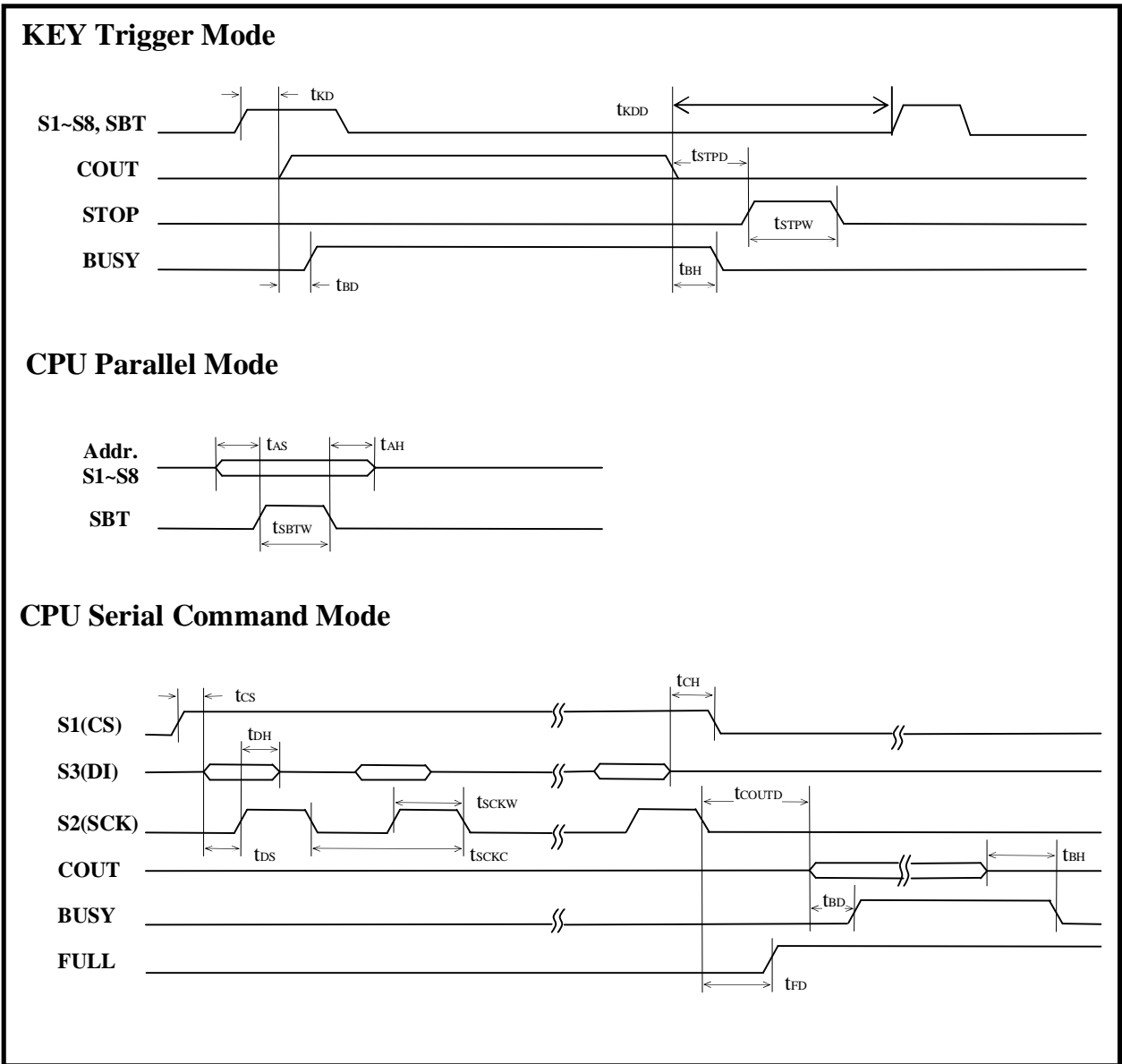
Fig. 18 Timing Waveform
